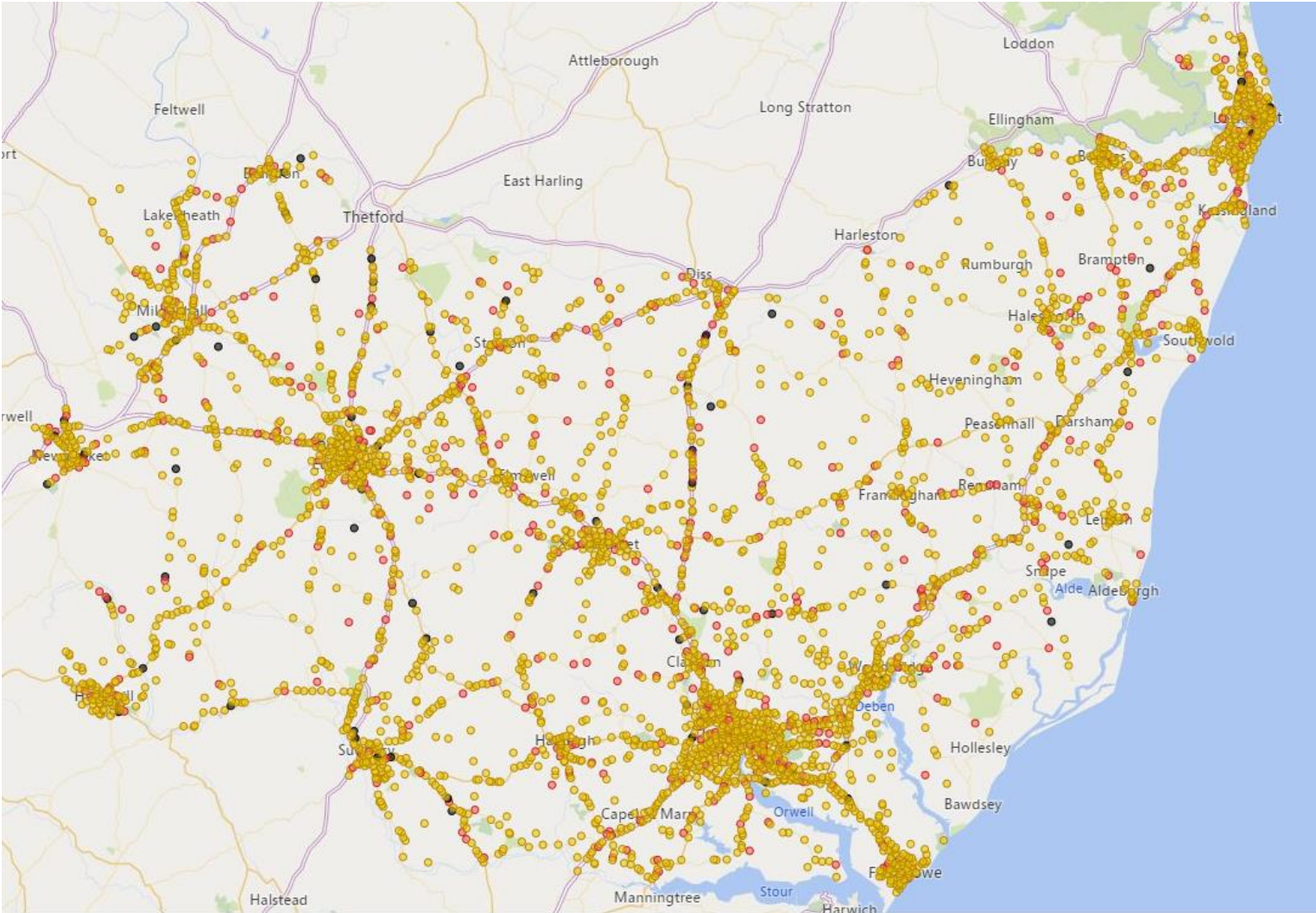
Collision Locations 2018
